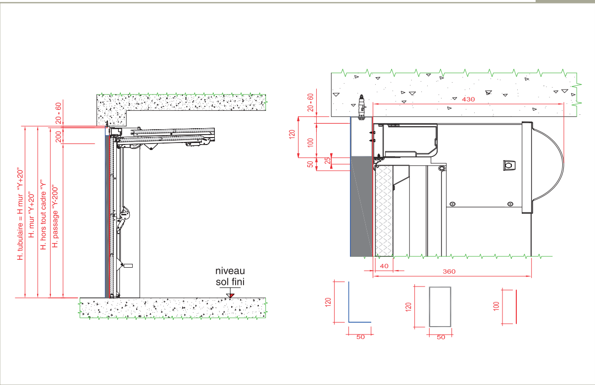
Coupe verticale - general
